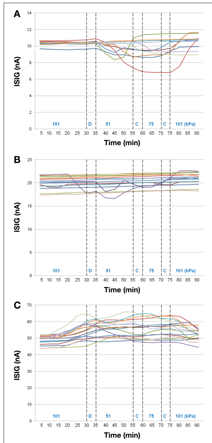
Figure 4. Input signal insulin glucose generated by each sensor in all three glucose concentrations: low/52 mg/dl (A), medium/88 mg/dl (B), and high/207 mg/dl (C) during the hypobaric test.
